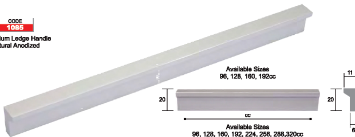
CODE 1166 Aluminium Railway Handle Natural Anodized
